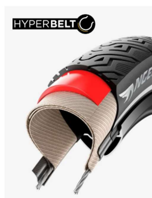
HYPERBELT The special construction dedicated to urban bikes made of a cut-resistant Nylon carcass paired with a 5mm layer of rubber for extra puncture protection
