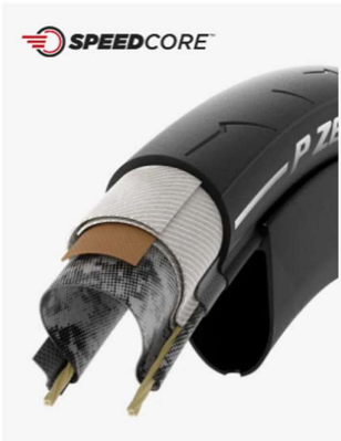
SPEEDCORE Cutting-edge TLR 120 tpi casing technology with an inner layer of aramid compound plus an aramid breaker
