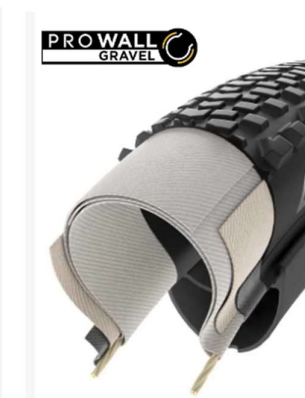
PROWALL GRAVEL The 60 tpi tubeless-ready gravel-specific construction; with sidewall protection meant to resist later cuts on different surfaces.
